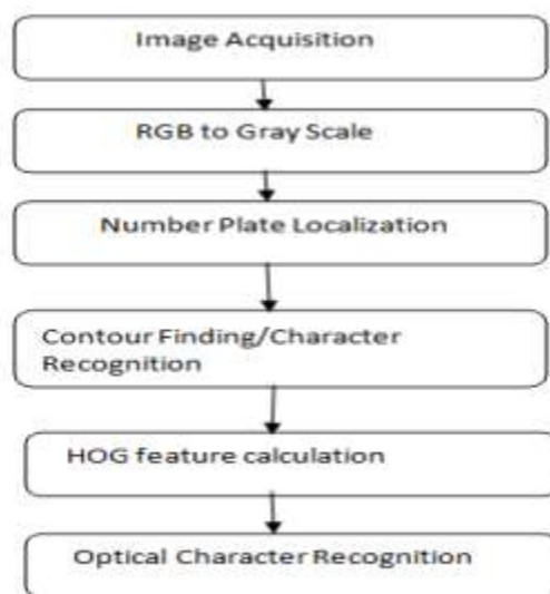
Fig 2: Block Diagram for the Proposed Algorithm
