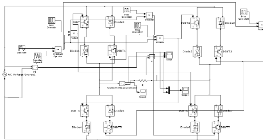
Fig. 10: Simulation circuit of 100Hz matrix converter
