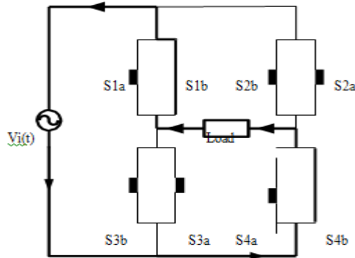
Fig. 5: State 2 negative cycle
