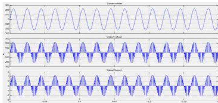
Fig. 13: MLS Simulation of SPMC with f_r=50 hz supply voltage, O/P Voltage, O/P Current
