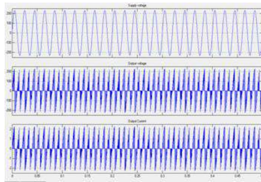
Fig. 14: MLS Simulation of SPMC with f_r=100 hz supply voltage, O/P Voltage, O/P Current
