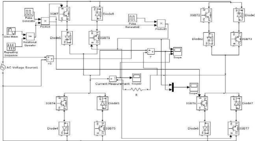
Fig. 9: Simulation circuit of 50Hz matrix converter
