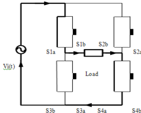
Fig. 4: State 1 positive cycle
