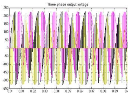
Fig. 15: Three phase output voltage waveforms
