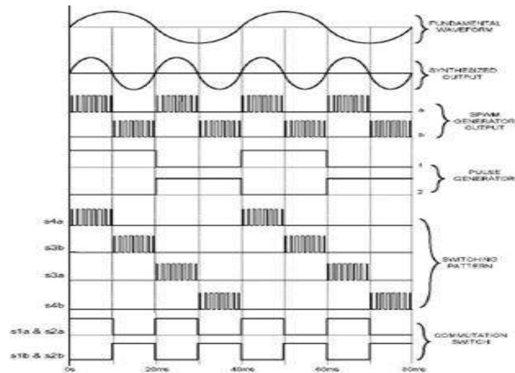
Fig. 12: Switching Pattern Generator (100 Hz)
