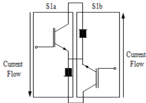
Fig 2: Bidirectional switch module (common emitter) III. SINUSOIDAL PULSE WIDTH MODULATION (SPWM)
