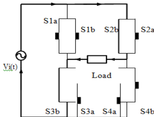
Fig. 6: State 3 positive cycle
