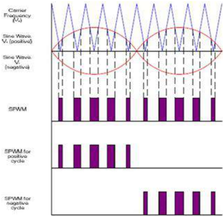
Fig. 3: Formation of SPWM
