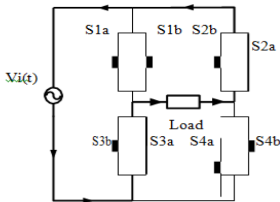
Fig. 7: State 4 negative cycle
