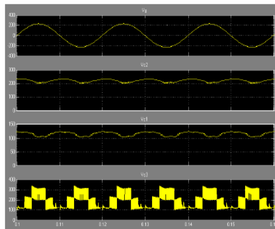
Fig:waveforms on DC side of seven level inverter
