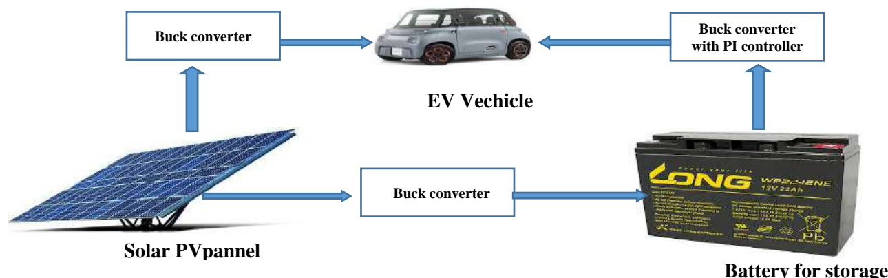
Fig 1: Block diagram representation of EV charging station
