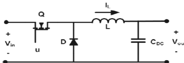
Fig 5: Representing buck converter
