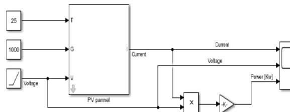
Fig4:Representation of PV cell in Simulink
