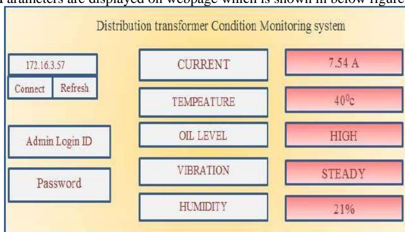
Fig.7. Distribution transformer condition monitoring system displaying on webpage
