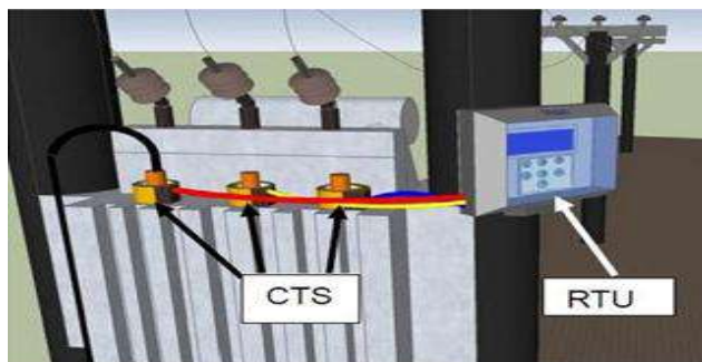
Fig.1. Distribution transformer condition monitoring hardware set up design
