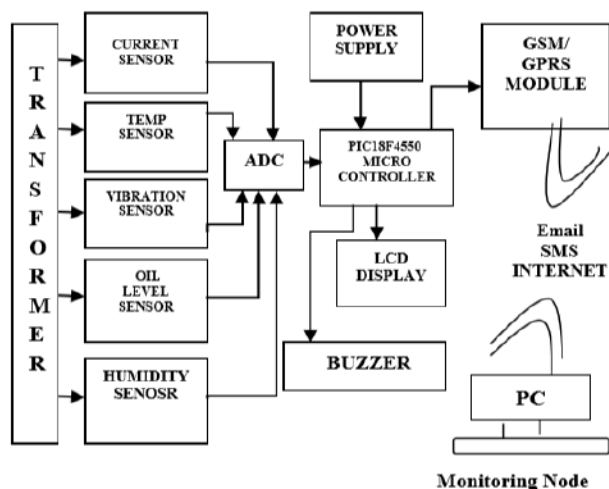
Fig.2. Block diagram of distribution transformer monitoring system
