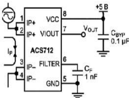
Fig.4. ACS712 IC with basic connections.
