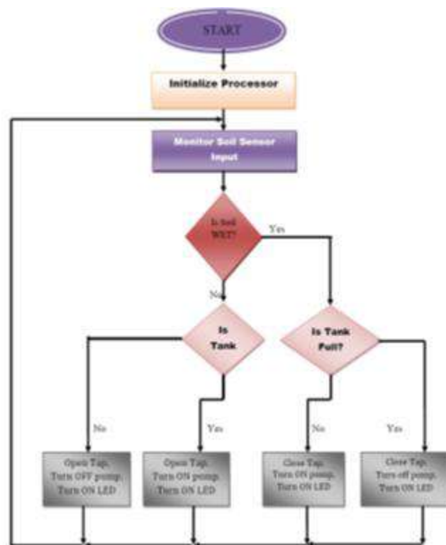
Figure.4.Flow chart of program excuted by Microcontroller
